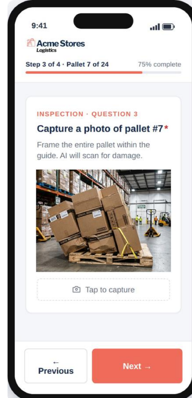
Defect Detection
