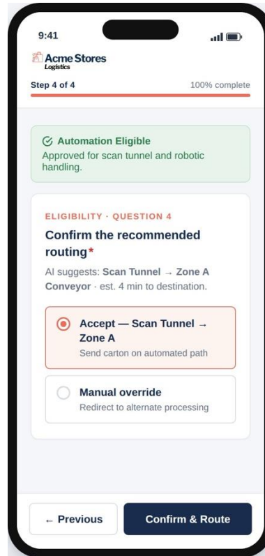
Automation Eligibility
